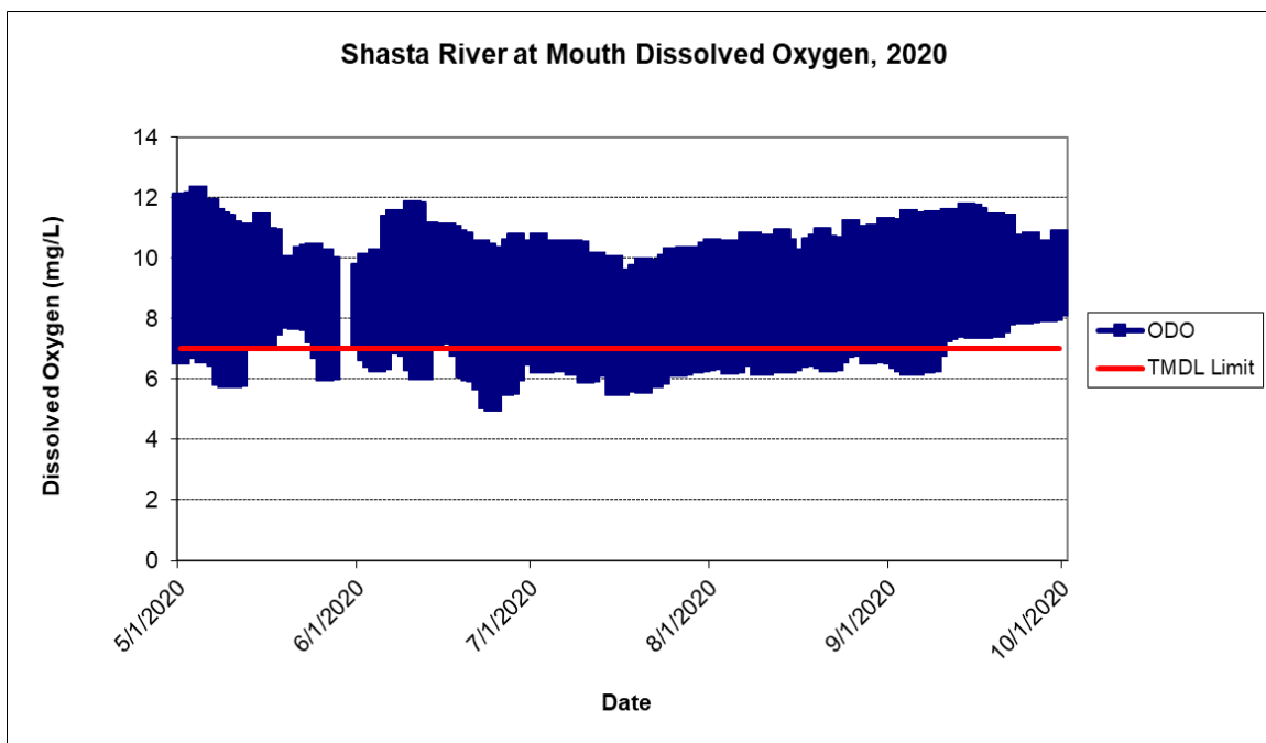
Figure 20. Instantaneous dissolved oxygen recorded every 15-minutes for the mouth of the Shasta River (SH) in 2020. The red line indicates the NCRWQCB Basin Plan site specific dissolved oxygen water quality objective for Shasta River, >7mg/L.
