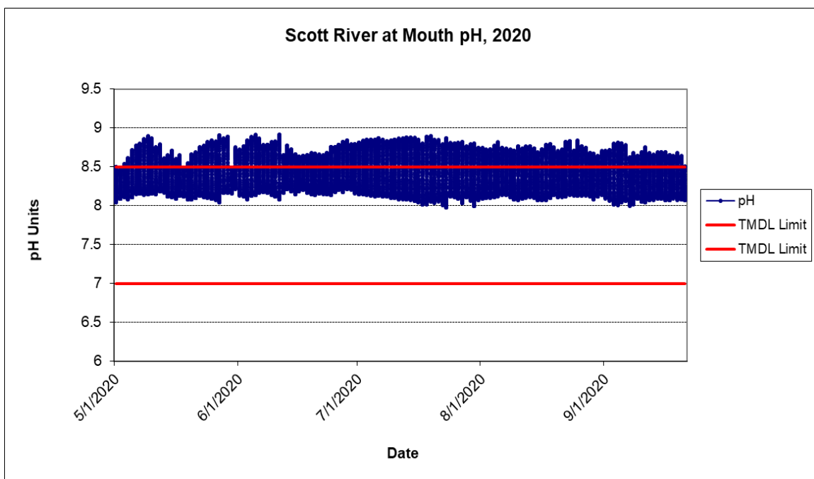
Figure 29. Instantaneous pH readings recorded every 15-minutes for the mouth of the Scott River (SC) in 2020. The red line indicates the NCRWQCB Basin Plan pH water quality objective for Scott River, 7 < X < 8.5 .
