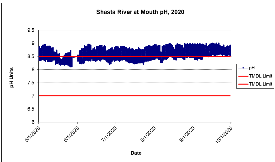
Figure 27. Instantaneous pH readings recorded every 15 minutes for the mouth of the Shasta River (SH) in 2020. The red line indicates the NCRWQCB Basin Plan pH water quality objective for Shasta River, 7 < X < 8.5 .
