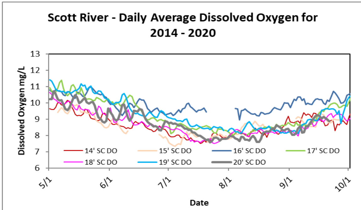
Figure 21. Daily average dissolved oxygen concentrations for the Scott River from 2014-2020.
