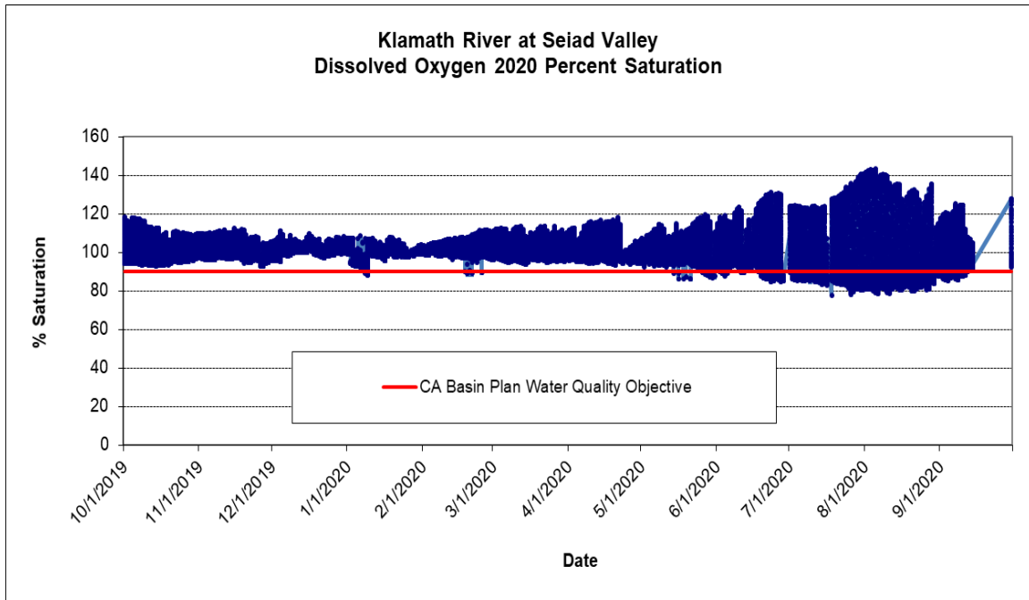
Figure 6. Percent saturation dissolved oxygen readings recorded every 15-minutes for Klamath River at Seiad Valley (SV) in 2020. The red line indicates the NCRWQCB Basin Plan Klamath River site specific dissolved oxygen water quality objective: from the mouth of the Scott River to Hoopa, >90% saturation year-round.
