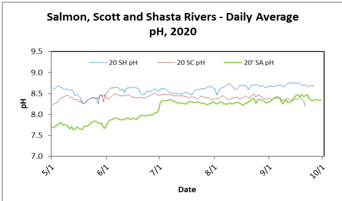
Figure 25. Daily average pH for Scott, Shasta, and Salmon Rivers, 2020.
