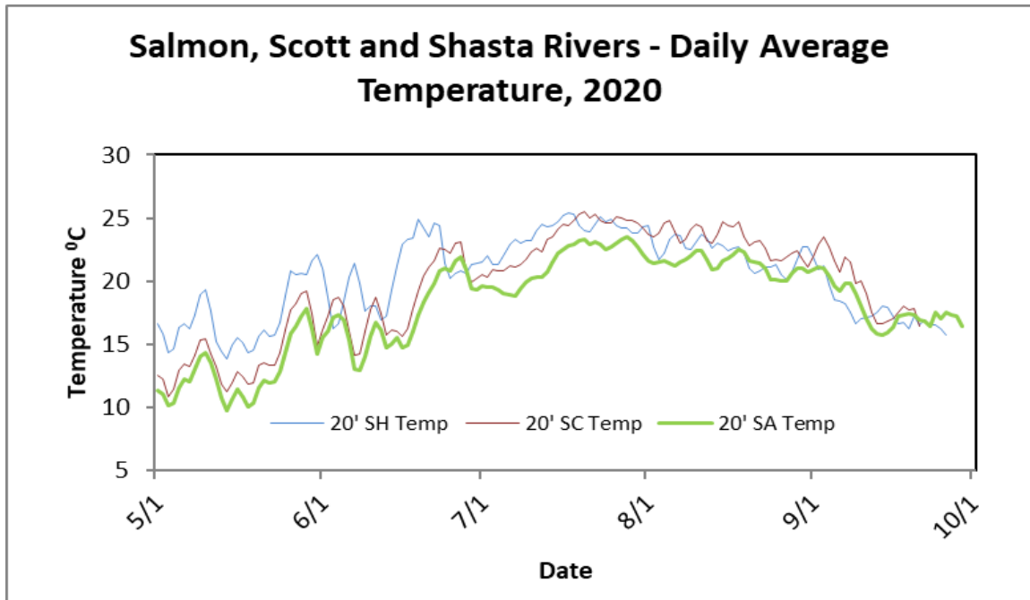
Figure 14. Daily average water temperature for Scott, Shasta, and Salmon Rivers, 2020.
