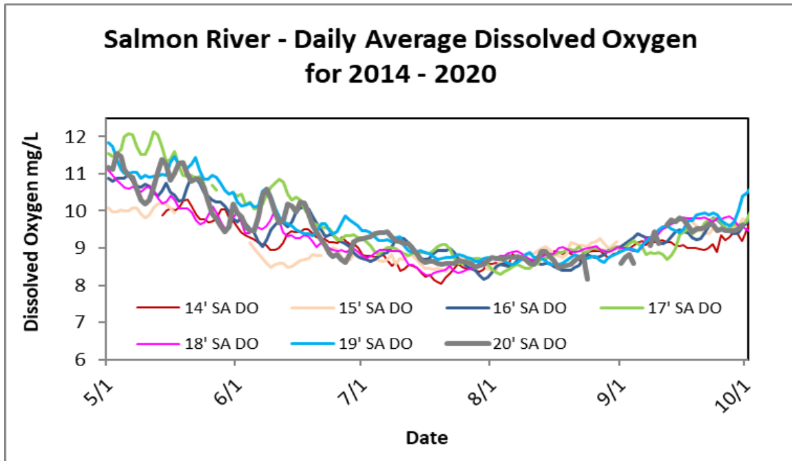
Figure 23. Daily average dissolved oxygen concentrations for the Salmon River from 2014-2020.
