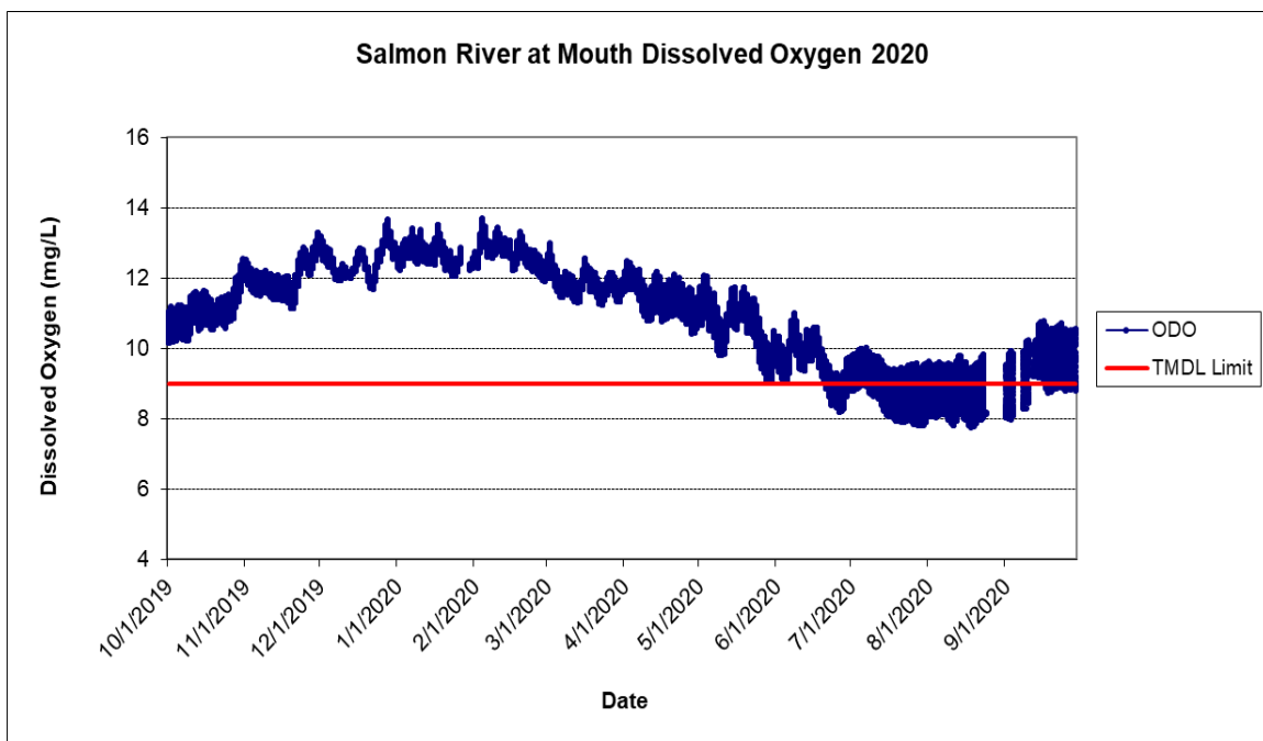
Figure 24: Instantaneous dissolved oxygen readings recorded every 15 minutes for the mouth of the Salmon River (SA) in 2020. The red line indicates the NCRWQCB Basin Plan site specific dissolved oxygen water quality objective for Salmon River, >9mg/L.
