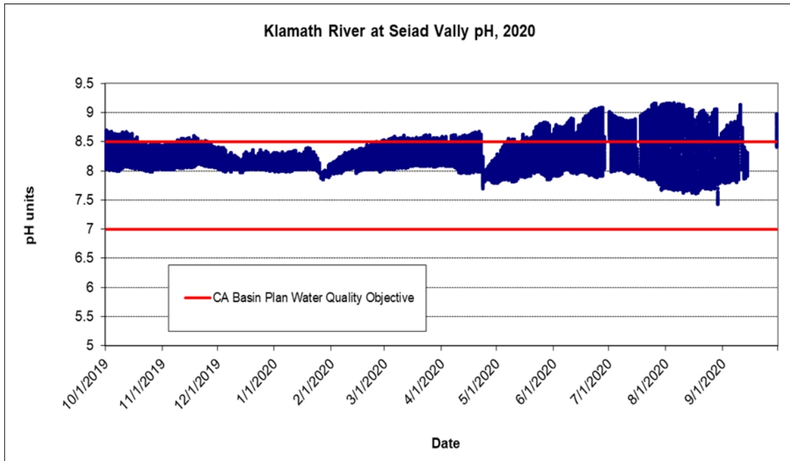
Figure 11. Instantaneous pH readings recorded every 15-minutes for Klamath River below Seiad Valley (SV) in 2020. The red lines are the NCRWQCB Basin Plan water quality objectives for the Klamath River, 7 < X < 8.5
