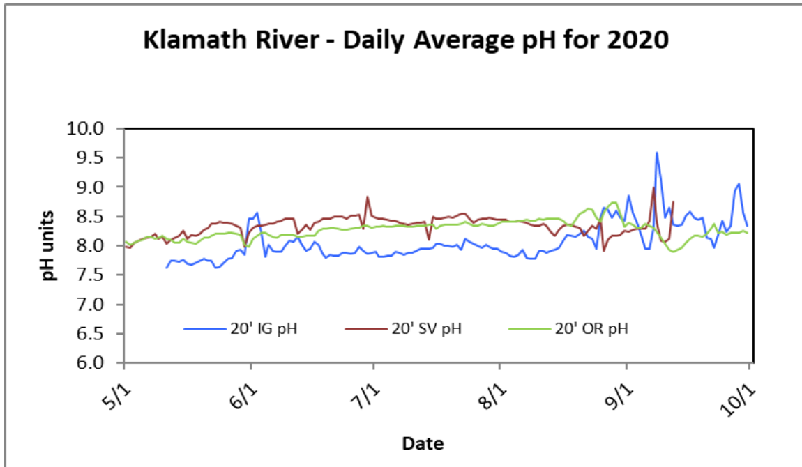
Figure 9. Daily average pH levels for 3 main stem Klamath River sites in 2020: below Iron Gate dam (IG), Seiad Valley (SV), and Orleans (OR).
