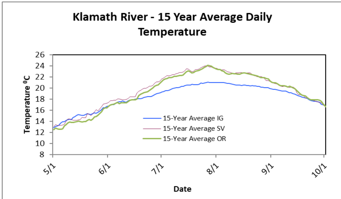
Figure 3. Averaged daily temperature from 2006-2020 at main stem Klamath River sites: below Iron Gate dam (IG), Seiad Valley (SV), and Orleans (OR).
