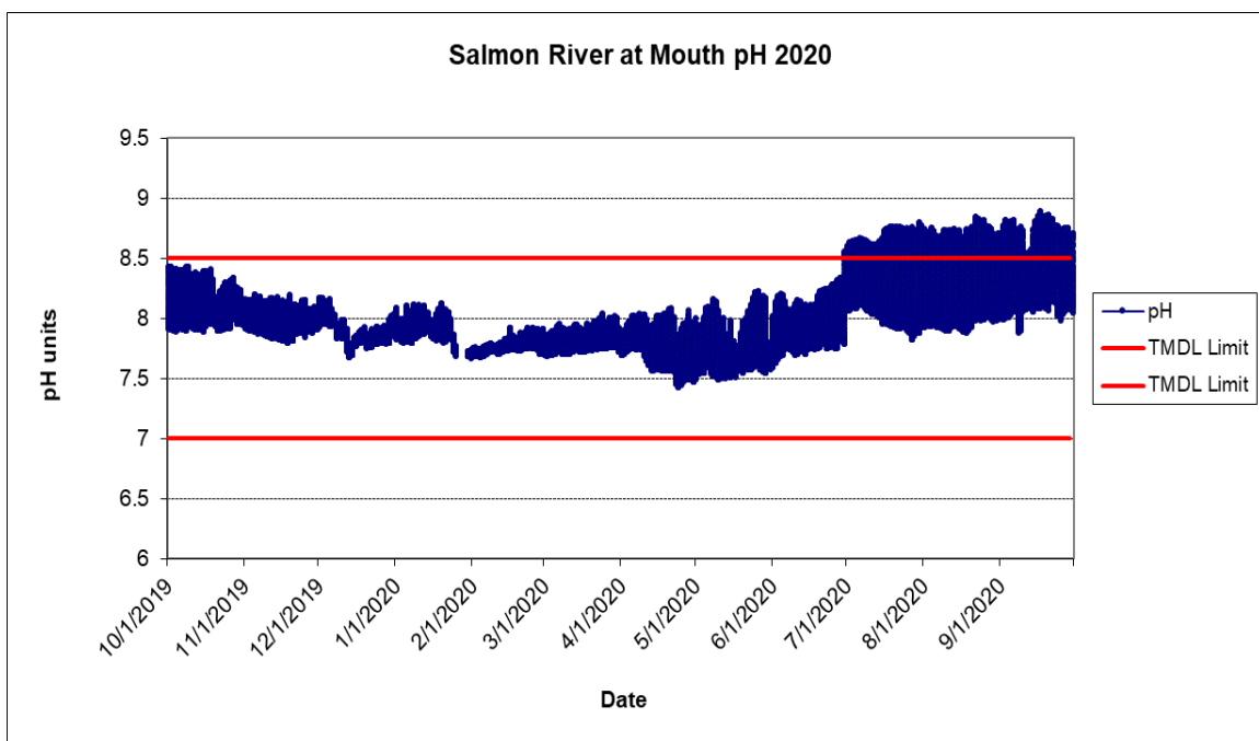
Figure 31. Instantaneous pH readings recorded every 15 minutes for the mouth of the Salmon River (SA) in 2020. The red line indicates the NCRWQCB Basin Plan pH water quality objective for Salmon River, 7 < X < 8.5 .
