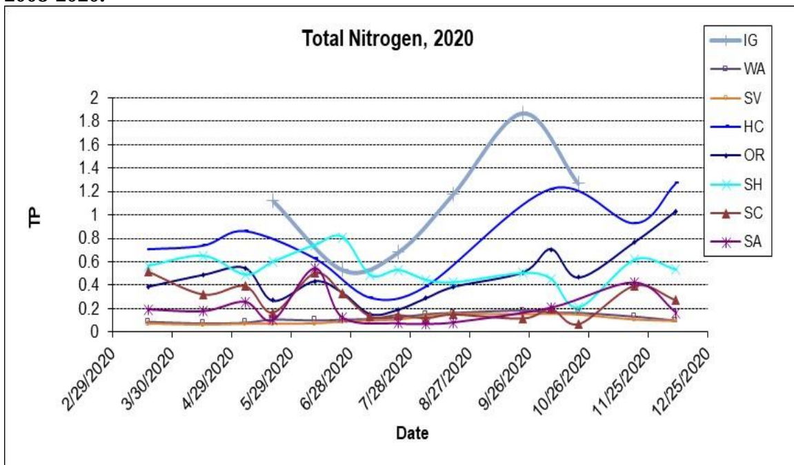
Figure 36. Total Nitrogen measured in mg/L for all monitored sites during 2020.
