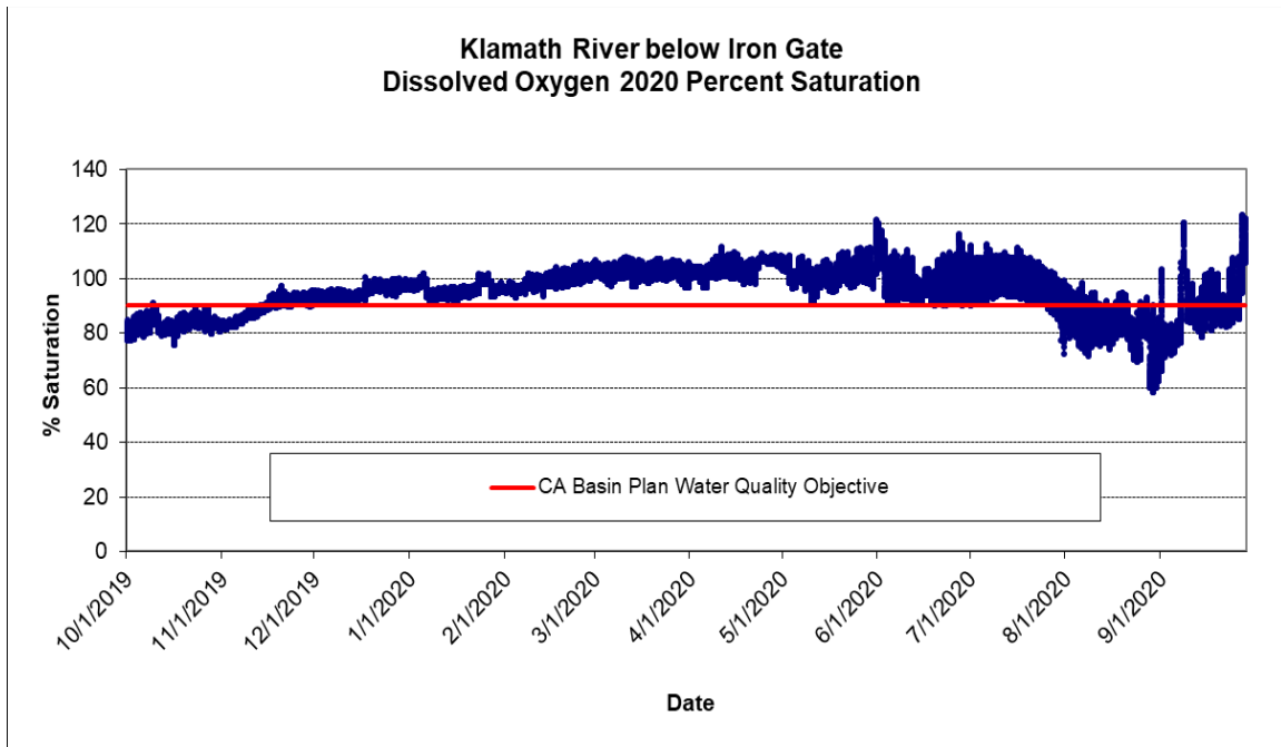
Figure 7. Percent saturation dissolved oxygen readings recorded every 15-minutes for Klamath River below Iron Gate Dam (IG) in 2020. The red line indicates the NCRWQCB Basin Plan Klamath River site specific dissolved oxygen water quality objective from Stateline (OR/CA) to the mouth of the Scott River, >90% saturation from Oct 1- March 30 and >85% from April 1-Sept 30.
