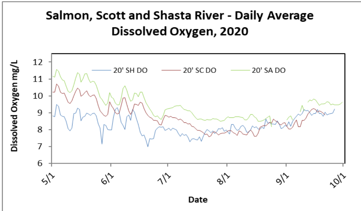
Figure 18. Daily average dissolved oxygen for Salmon, Scott and Shasta River, 2020.
