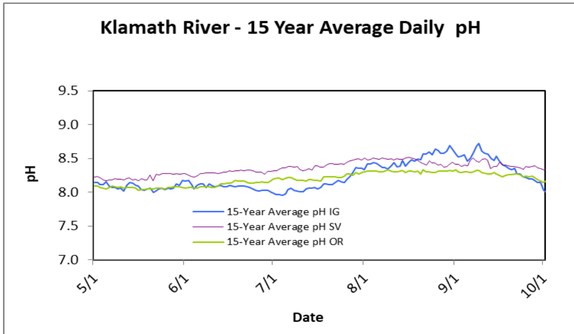
Figure 13. Daily average pH, 2006-2020 at main stem Klamath River sites: below Iron Gate dam (IG), Seiad Valley (SV), and Orleans (OR).
