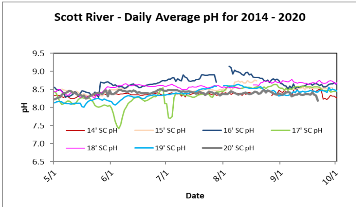
Figure 28. Daily average pH concentrations for the Scott River from 2014-2020.
