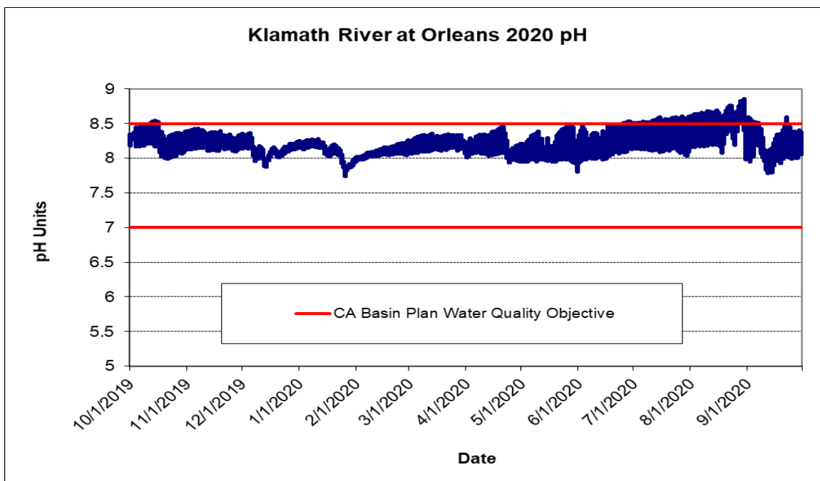
Figure 10. Instantaneous pH readings recorded every 15-minutes for Klamath River at Orleans (OR) in 2020. The red lines are the NCRWQCB Basin Plan water quality objectives for the Klamath River, 7 < X < 8.5 .
