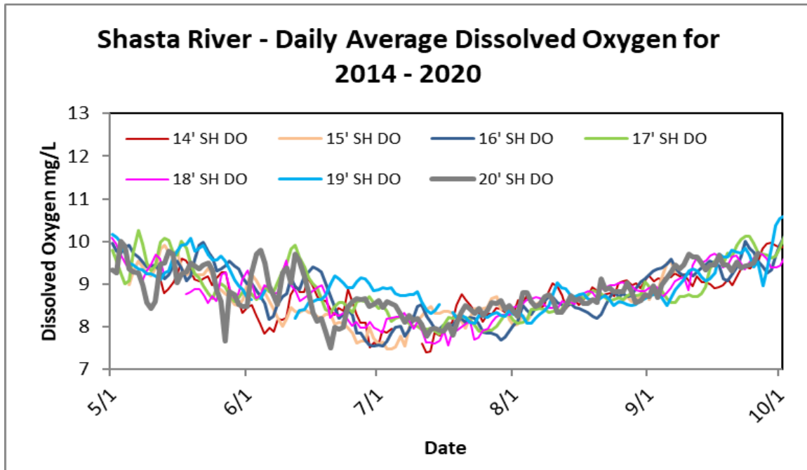
Figure 19. Daily average dissolved oxygen concentrations for the Shasta River from 2014-2020.
