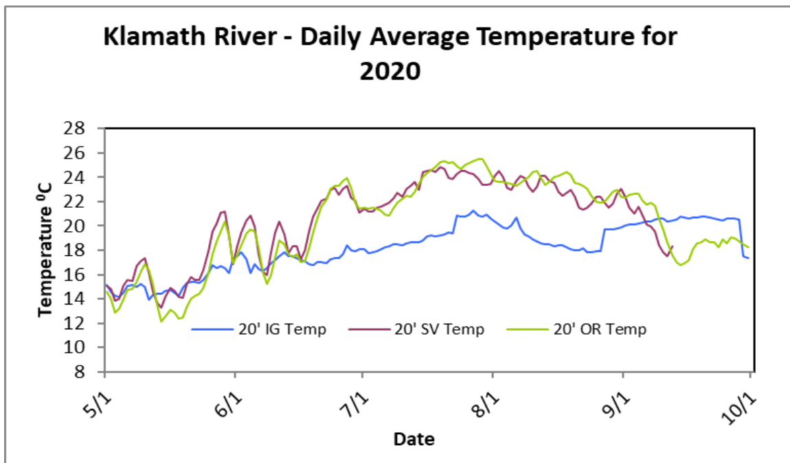
Figure 2. Daily average temperatures for 3 main stem Klamath River sites in 2020: below Iron Gate dam (IG), Seiad Valley (SV), and Orleans (OR).
