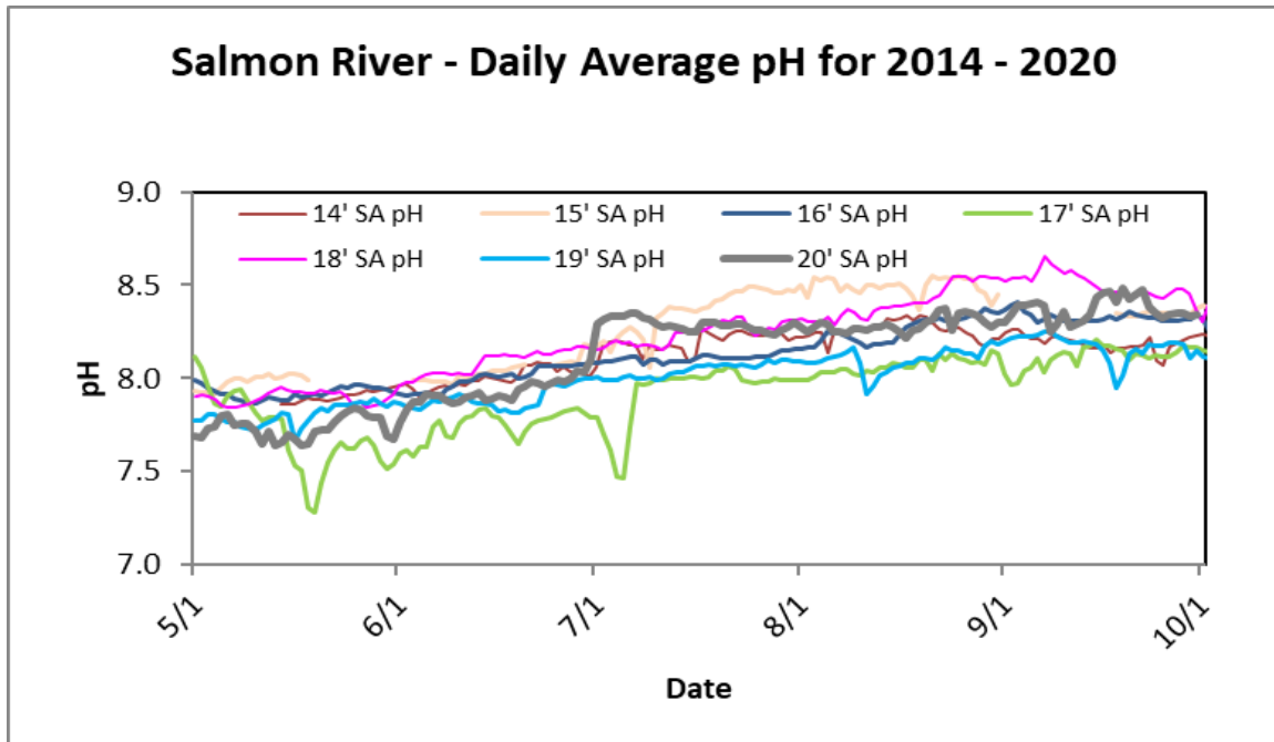
Figure 30. Daily average pH concentrations for the Salmon River from 2014-2020.
