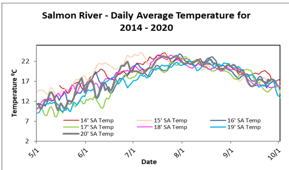
Figure 17. Daily average water temperatures for the Salmon River from 2014-2020.
