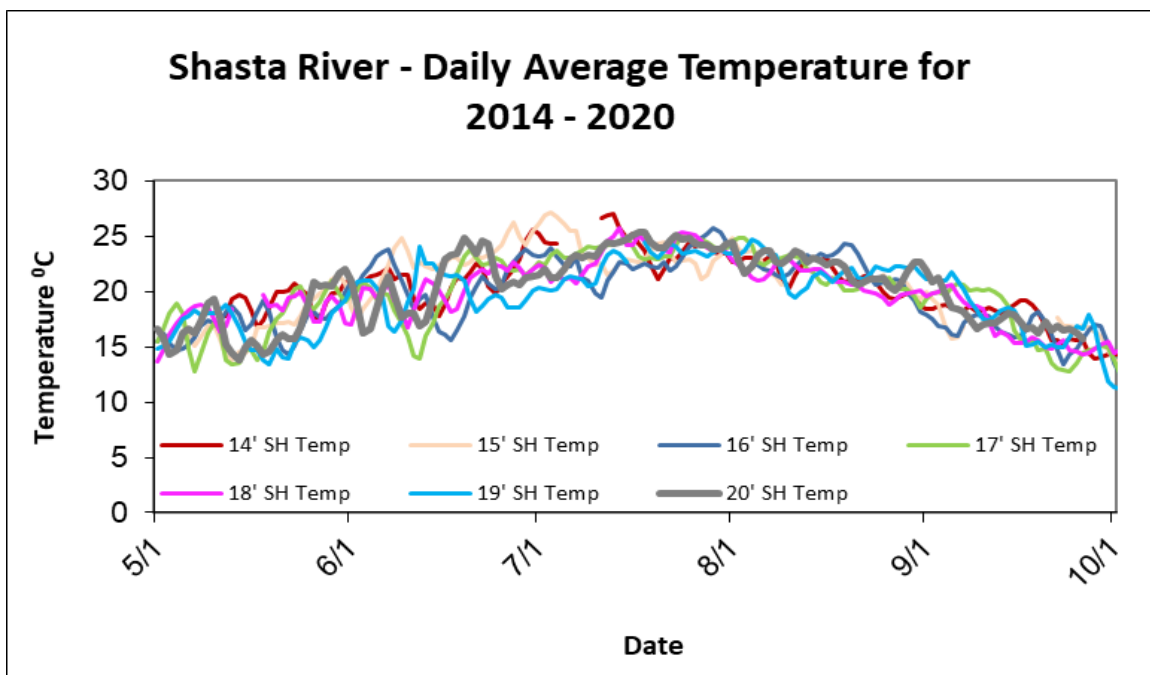
Figure 15. Daily average water temperatures for the Shasta River from 2014-2020.
