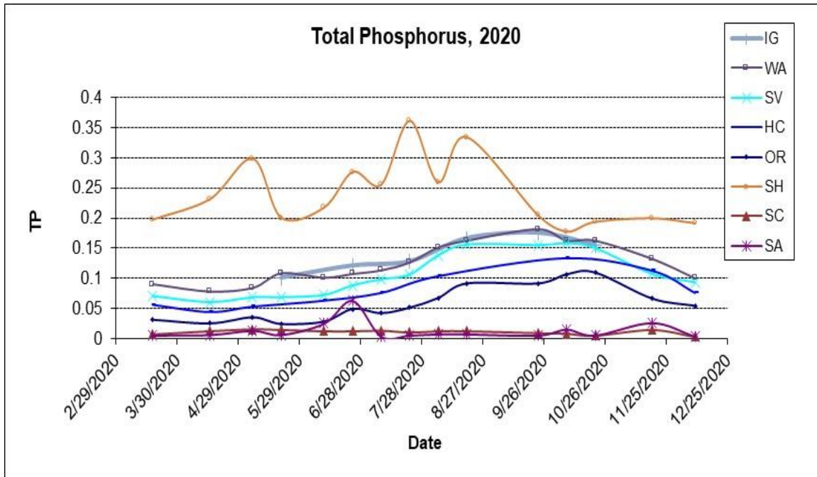
Figure 33. Total Phosphorus measured in mg/L for all monitored sites during 2020.
