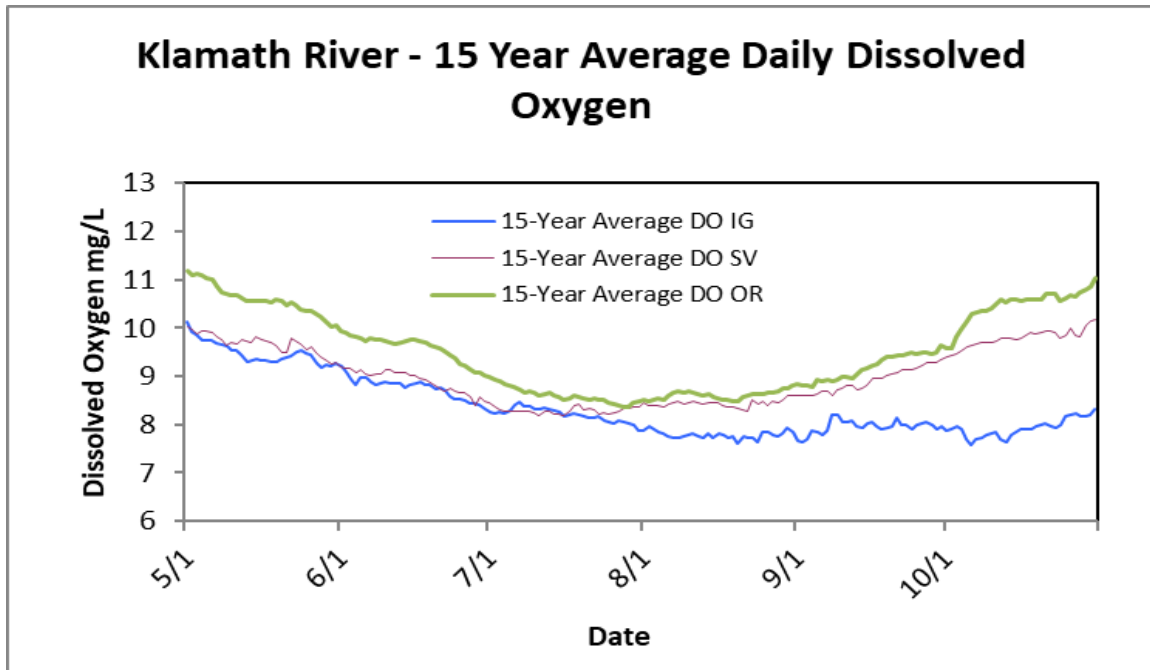
Figure 8. Average daily dissolved oxygen levels from 2006-2020 at main stem Klamath River sites: below Iron Gate dam (IG), Seiad Valley (SV), and Orleans (OR).
