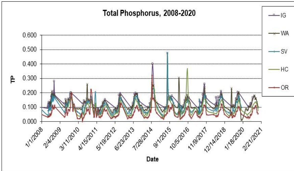
Figure 35. Total Phosphorus measured in mg/L for Klamath River sites during 2008-2020.
