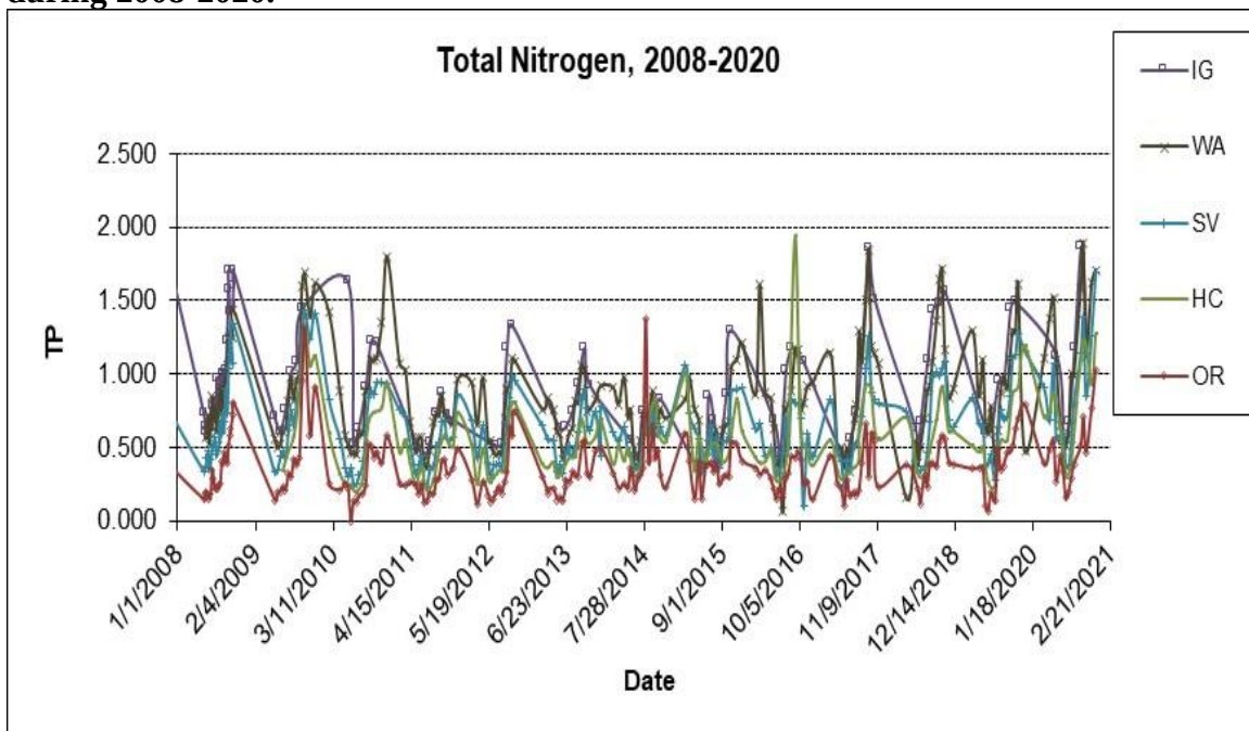
Figure 38. Total Nitrogen measured in mg/L for Klamath River during 2008-2020.
