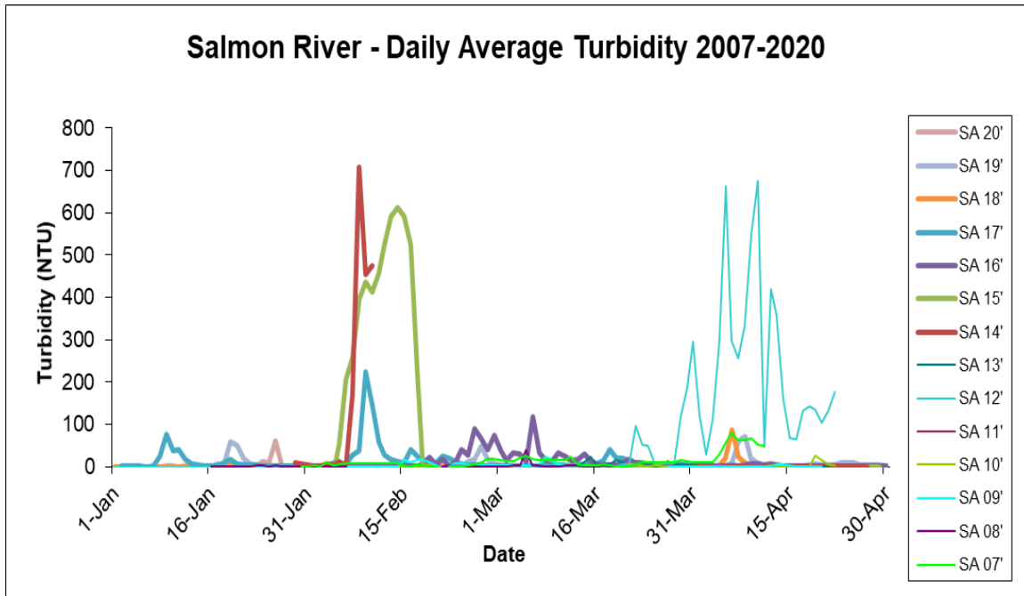
Figure 32. Daily average turbidity, winters of 2007 - 2020 on Salmon River (SA).
