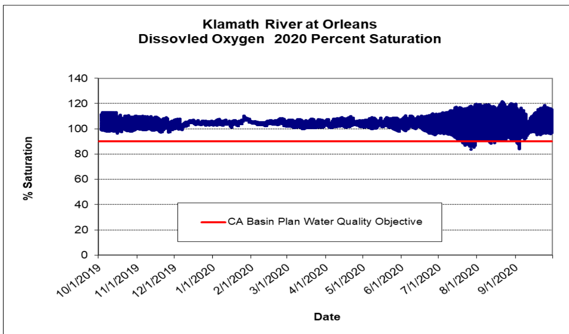
Figure 5. Percent saturation dissolved oxygen readings recorded every 15-minutes for Klamath River at Orleans (OR) in 2020. The red line indicates the NCRWQCB Basin Plan Klamath River site specific dissolved oxygen water quality objective: from the mouth of the Scott River to Hoopa, >90% saturation year-round.
