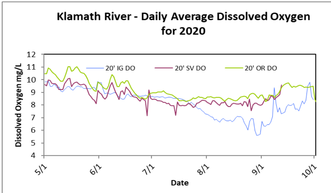
Figure 4. Daily average dissolved oxygen levels for 3 main stem Klamath River sites in 2020: below Iron Gate dam (IG), Seiad Valley (SV), and Orleans (OR).
