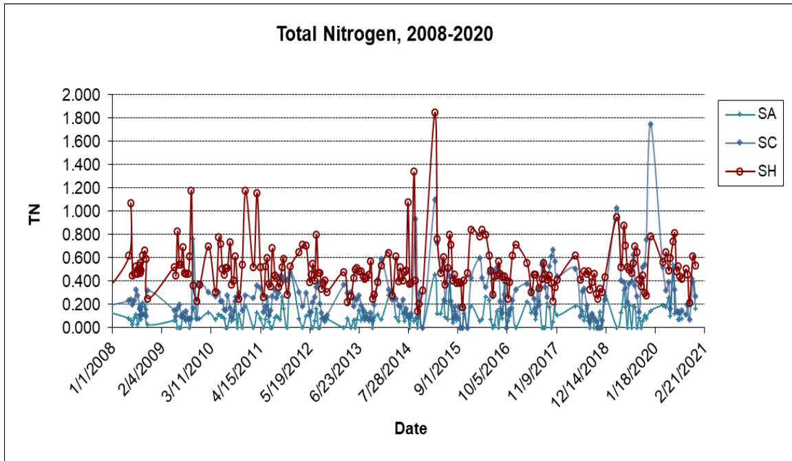
Figure 37. Total Nitrogen measured in mg/L for Salmon, Scott and Shasta Rivers during 2008-2020.
