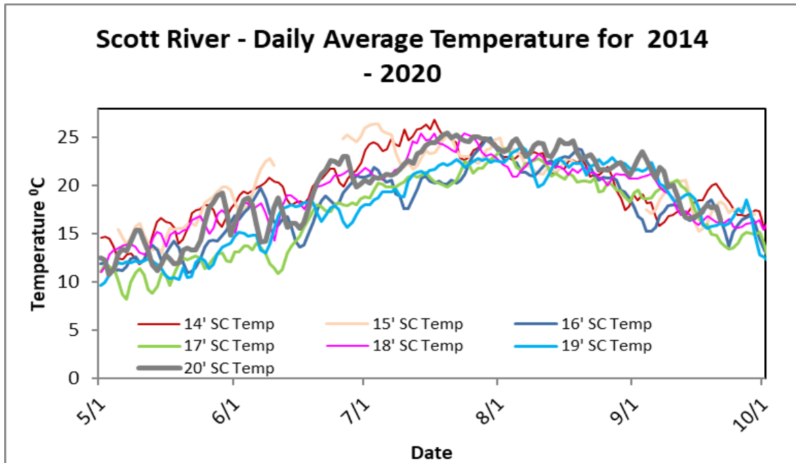
Figure 16. Daily average water temperatures for the Scott River from 2014-2020.
