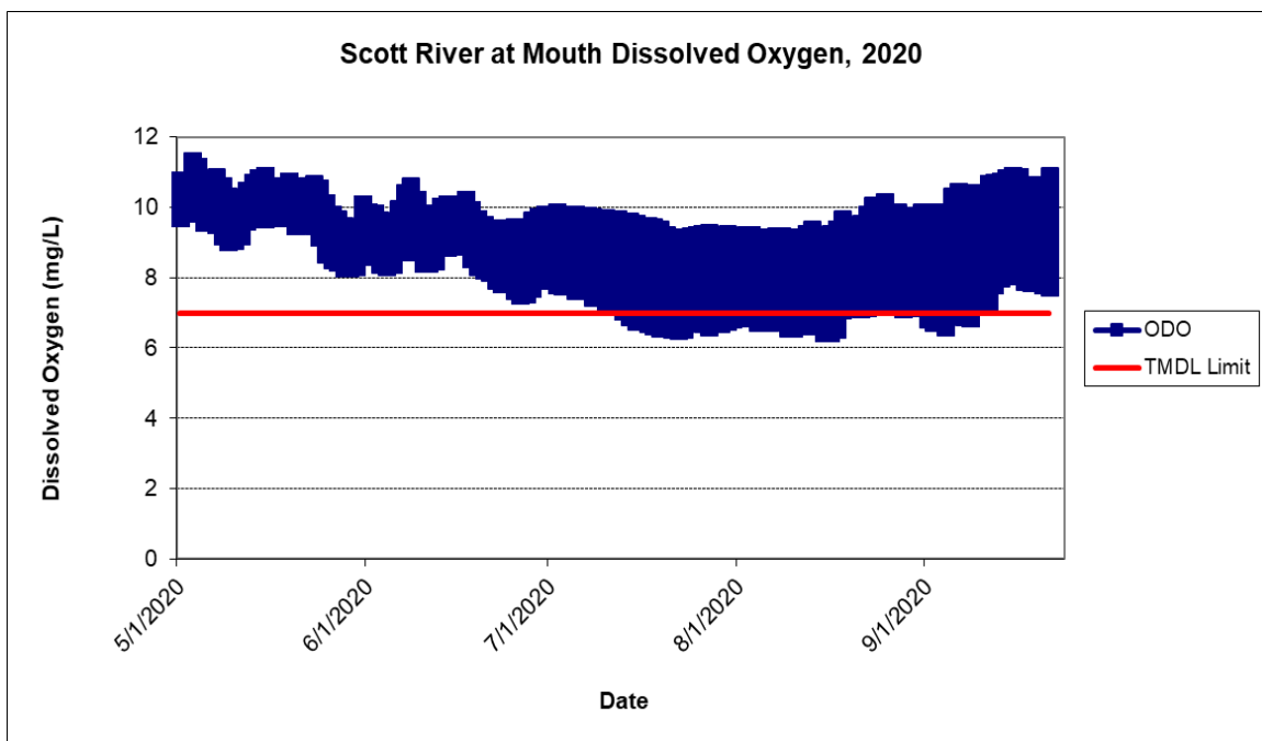
Figure 22. Instantaneous dissolved oxygen readings recorded every 15-minutes for the mouth of the Scott River (SC) in 2020. The red line indicates the NCRWQCB Basin Plan site specific dissolved oxygen water quality objective for Scott River, >7\text{mg/L} .
