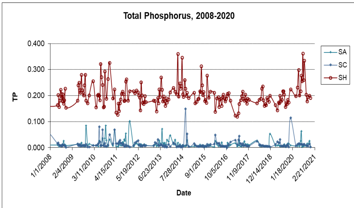
Figure 34. Total Phosphorus measured in mg/L for Salmon, Scott and Shasta Rivers sites during 2008-2020.
