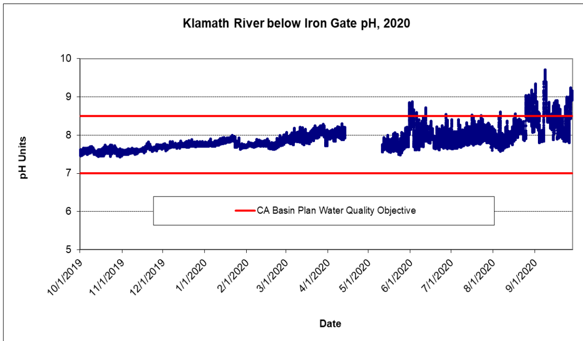
Figure 12. Instantaneous pH readings recorded every 15-minutes for Klamath River below Iron Gate (IG) in 2020. The red lines are the NCRWQCB Basin Plan water quality objectives for the Klamath River, 7 < X < 8.5
